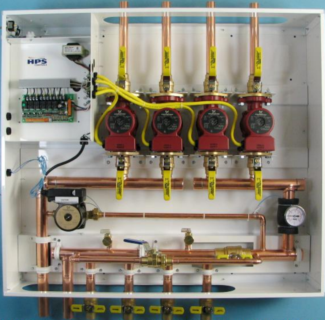
CFI-422 [Combo Temp Injection 2-Hi, 2-Lo Zone Control Station]
